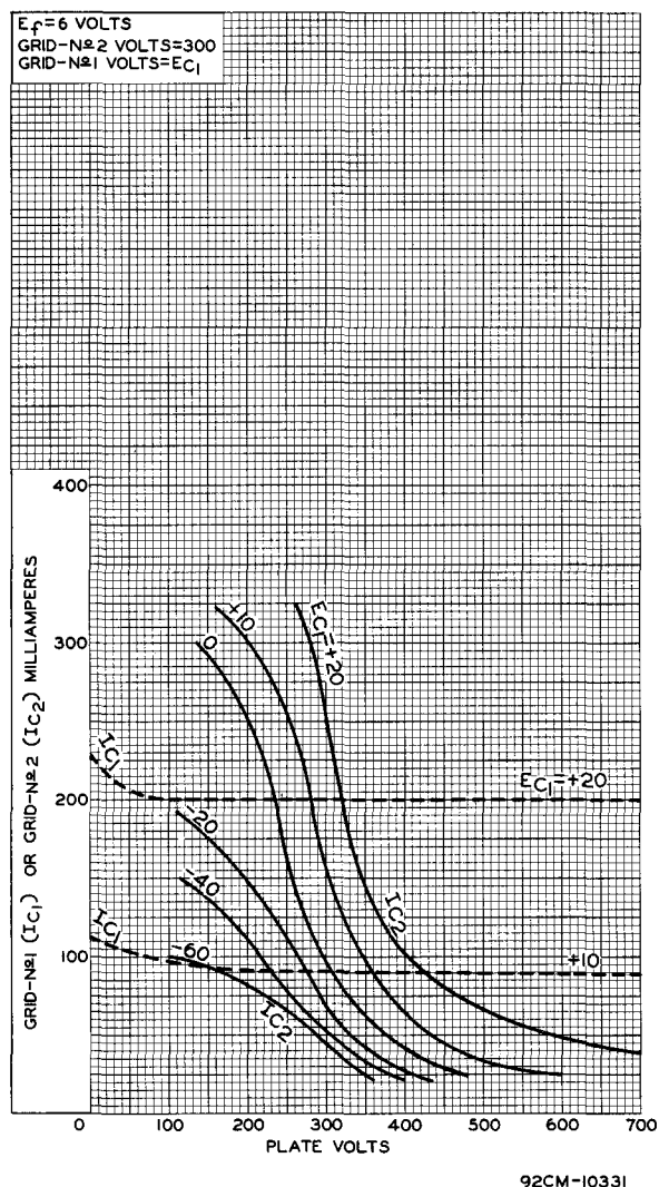
Fig. 2 - Typical Characteristics of Type 7580.
