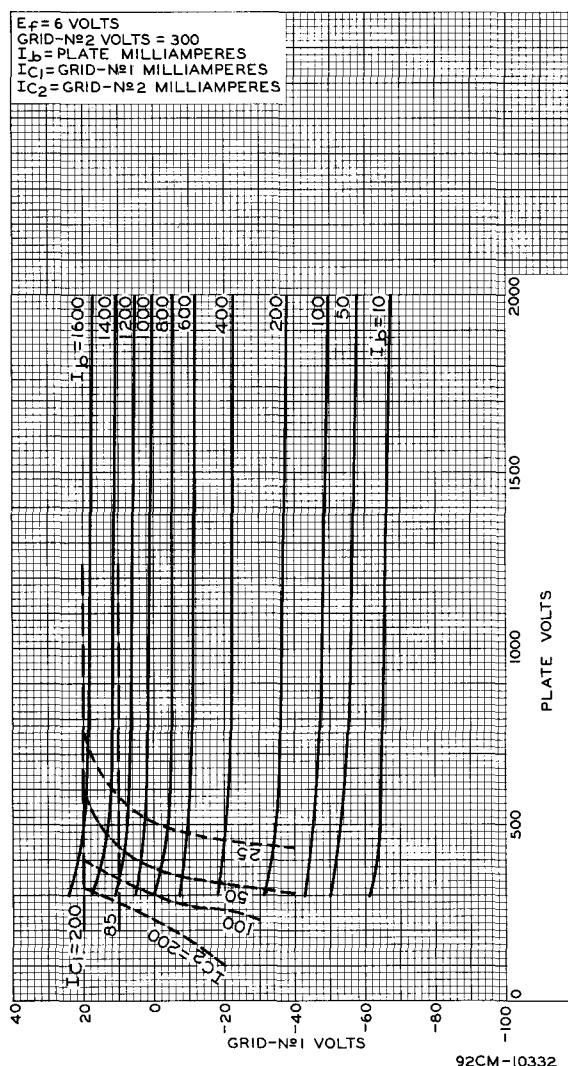
Fig. 3 - Typical Constant-Current Characteristics of Type 7580.
