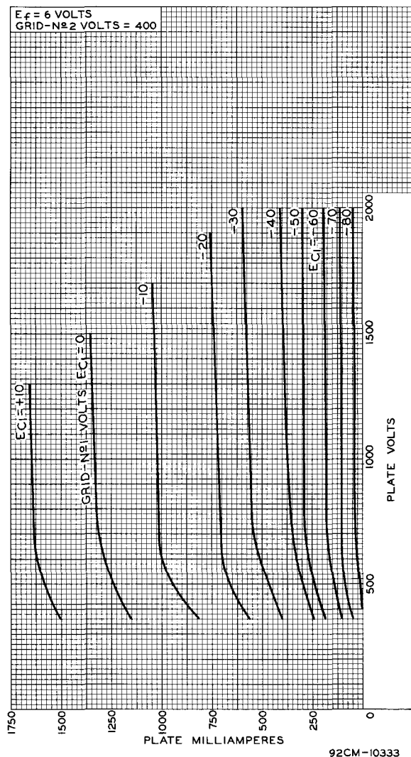
Fig. 4 - Typical Plate Characteristics of Type 7580.
