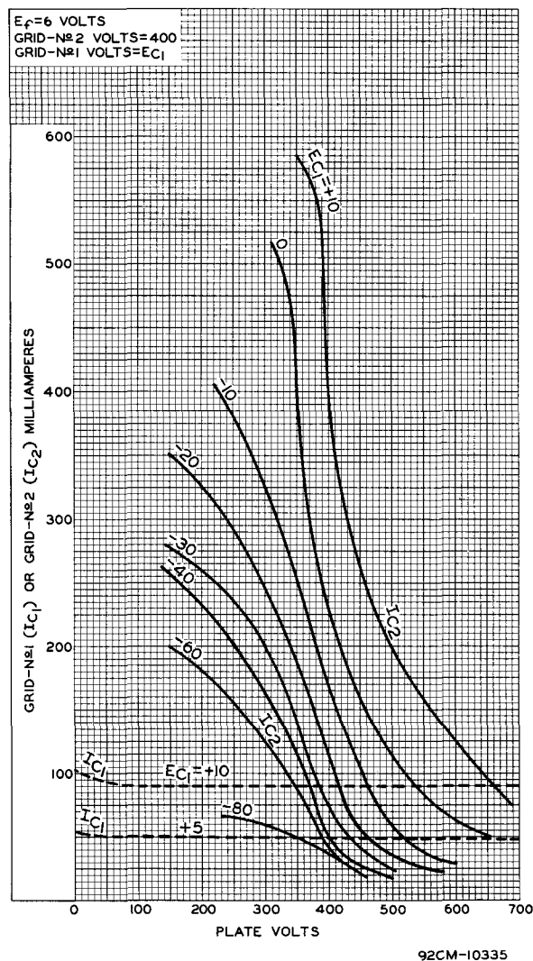
Fig. 5 - Typical Characteristics of Type 7580.
