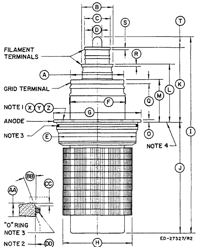
DETAIL OF RECOMMENDED OPENING IN COOLING JACKET
