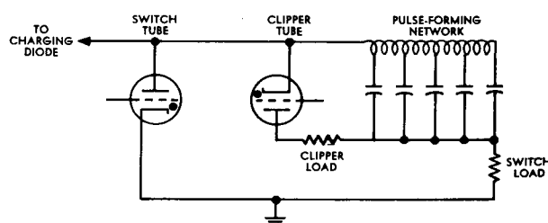
FIGURE 2. FRONT OF LINE CLIPPER
