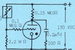
7401 ACTING AS A RELAY FOR A CADMIUM SULPHIDE PHOTO CELL
