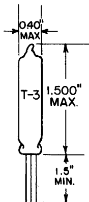
GLASS VIEW
