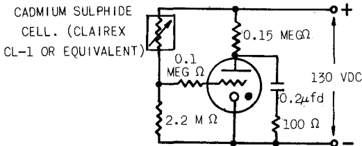
7401 ACTING AS A RELAY FOR A CADMIUM SULPHIDE PHOTO CELL
