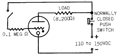
7401 USED AS A MECHANICALLY OPERATED RELAY
