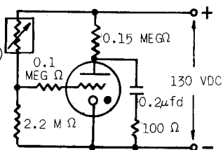
7400 ACTING AS A RELAY FOR A CADMIUM SULPHIDE PHOTO CELL
