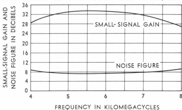
NOISE FIGURE AND SMALL-SIGNAL GAIN VS. FREQUENCY
