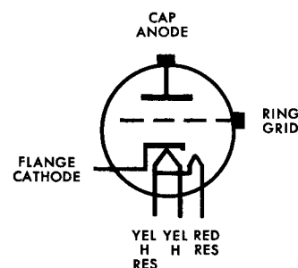
BASING DIAGRAM
