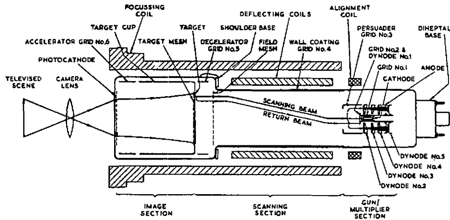
Fig. 1—Schematic Arrangement
