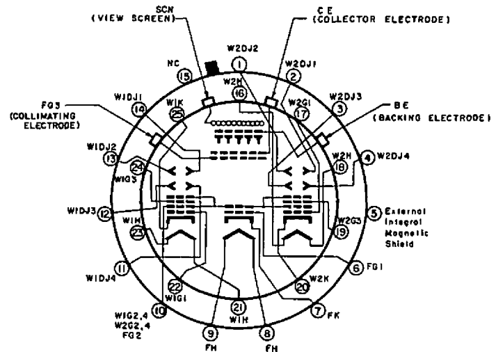
BOTTOM VIEW
