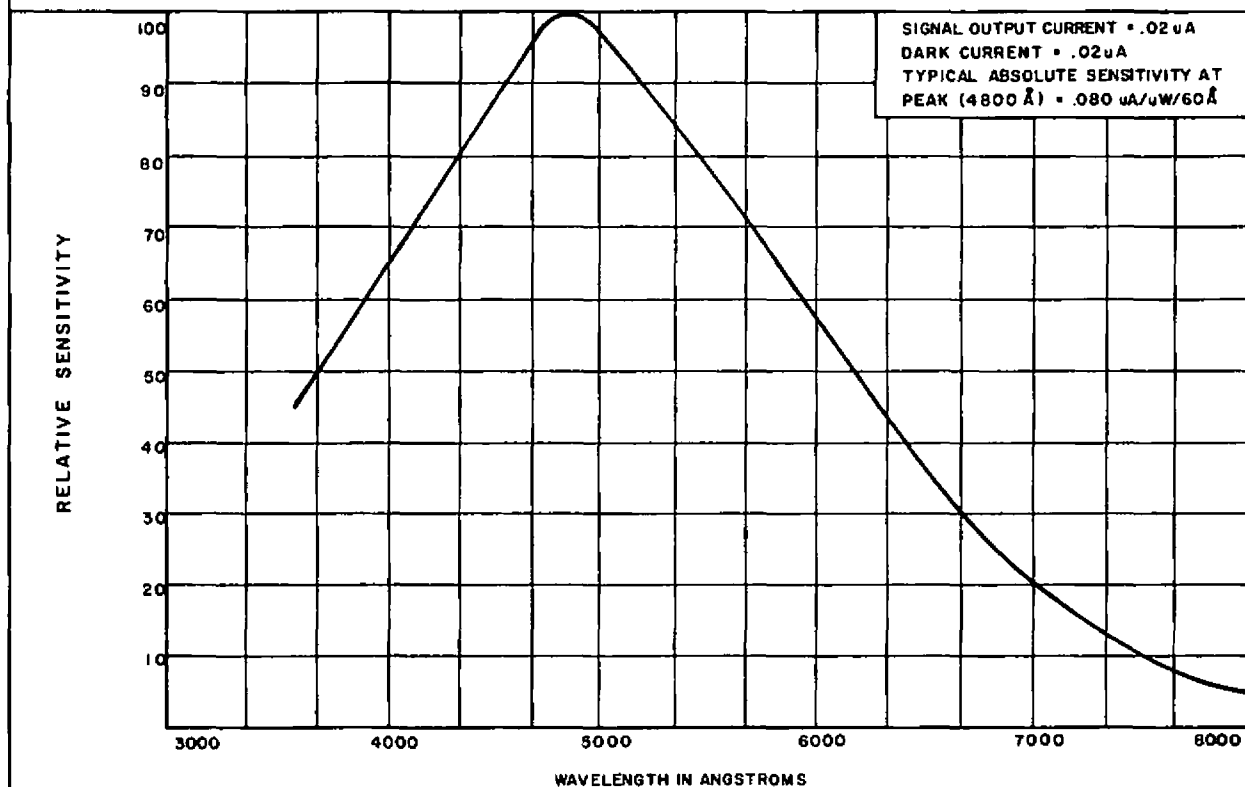
FIG. 4 SPECTRAL RESPONSE
