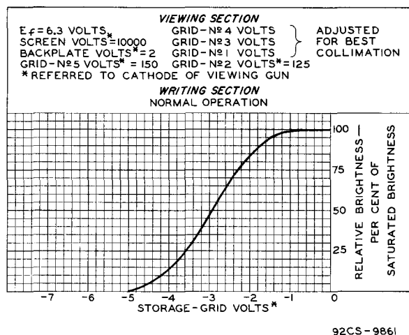
Fig.4 - Typical Storage-Grid Characteristic of Type 7315.
