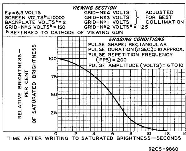
Fig.5 - Typical Erasure Characteristic of Type 7315.
