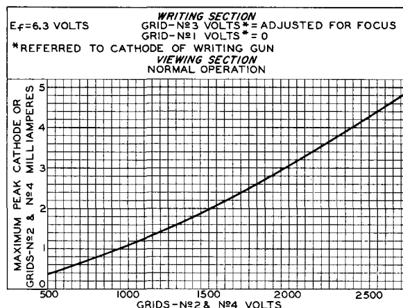
Fig.6 - Current Characteristic for Writing Gun of Type 7315.
