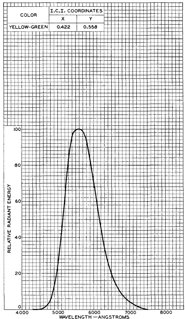
Fig.2 - Spectral-Energy Emission Characteristic of Phosphor P20 Used in Type 7315.
