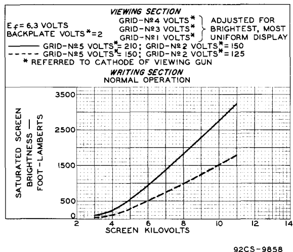
Fig.3 - Typical Characteristics of Type 7315.
