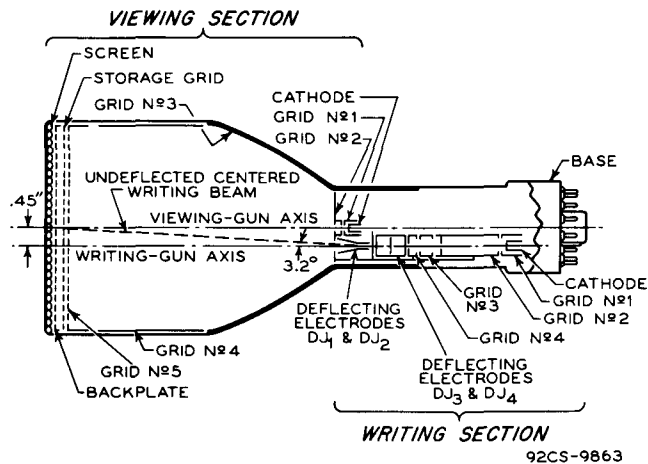
Fig.1 - Schematic Arrangement of Type 7315.
