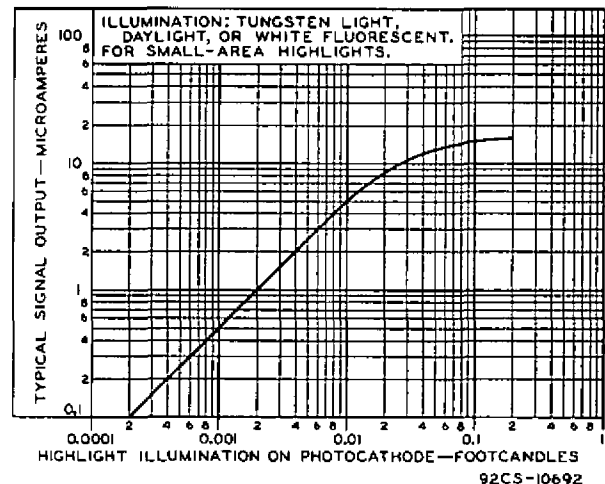
Fig. 3 - Basic Light Transfer Characteristic of Type 7295-A.
