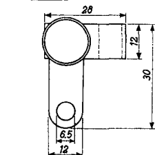
Heater connector 40634
