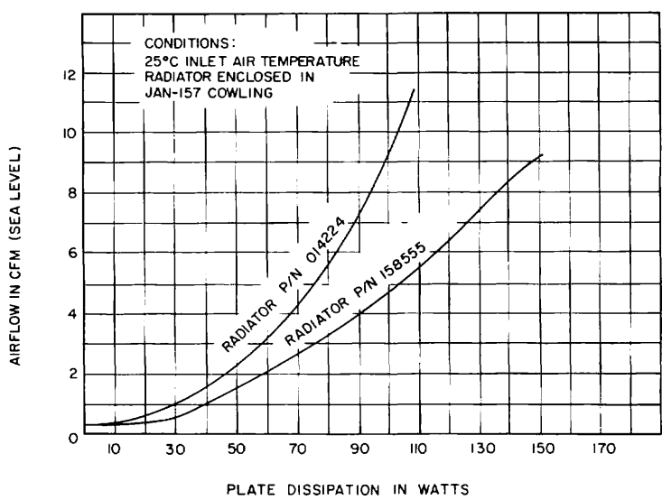
MAXIMUM PLATE DISSIPATION vs COOLING AIRFLOW
