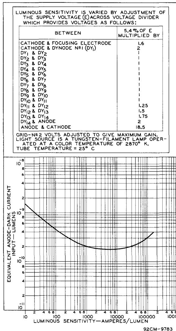
Fig. 3 - Typical Anode-Dark-Current Characteristic of Type 7265.
