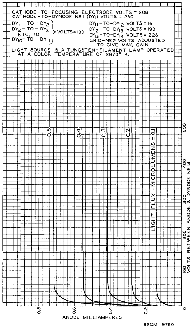
Fig. 2 - Average Anode Characteristics of Type 7265.
