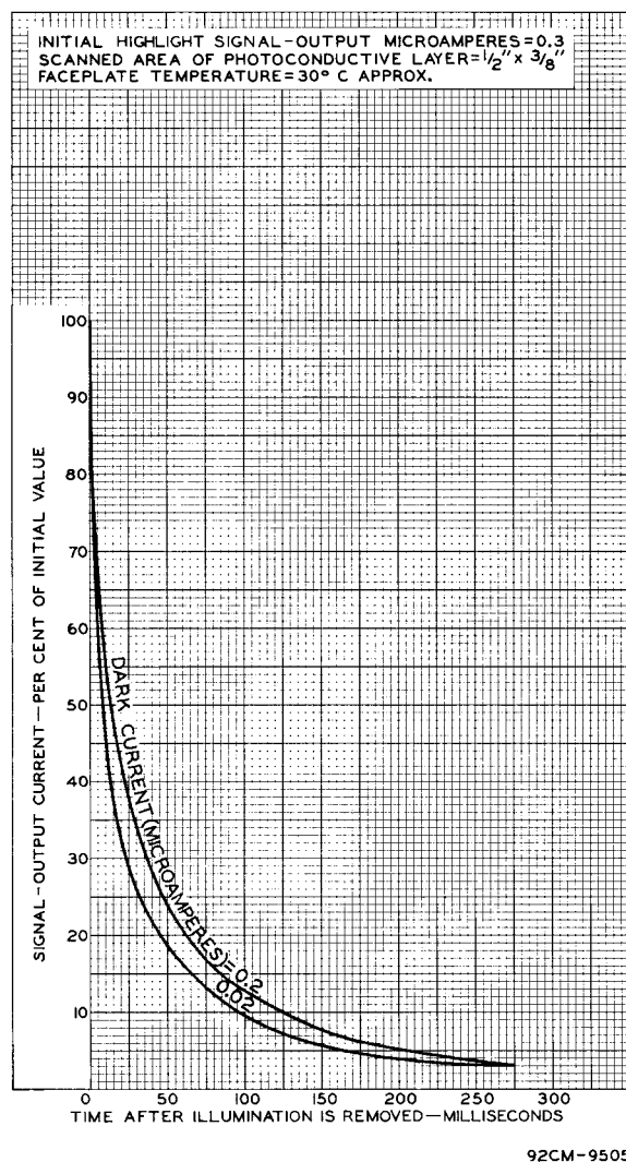
Fig. 10 - Typical Persistence Characteristics of Type 7262.
