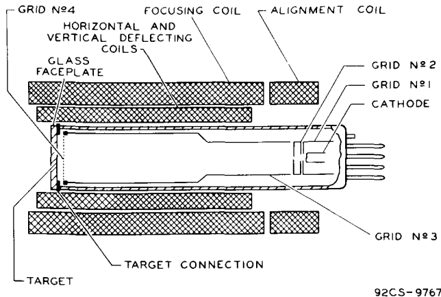
Fig. 1 - Schematic Arrangement of Type 7262.
