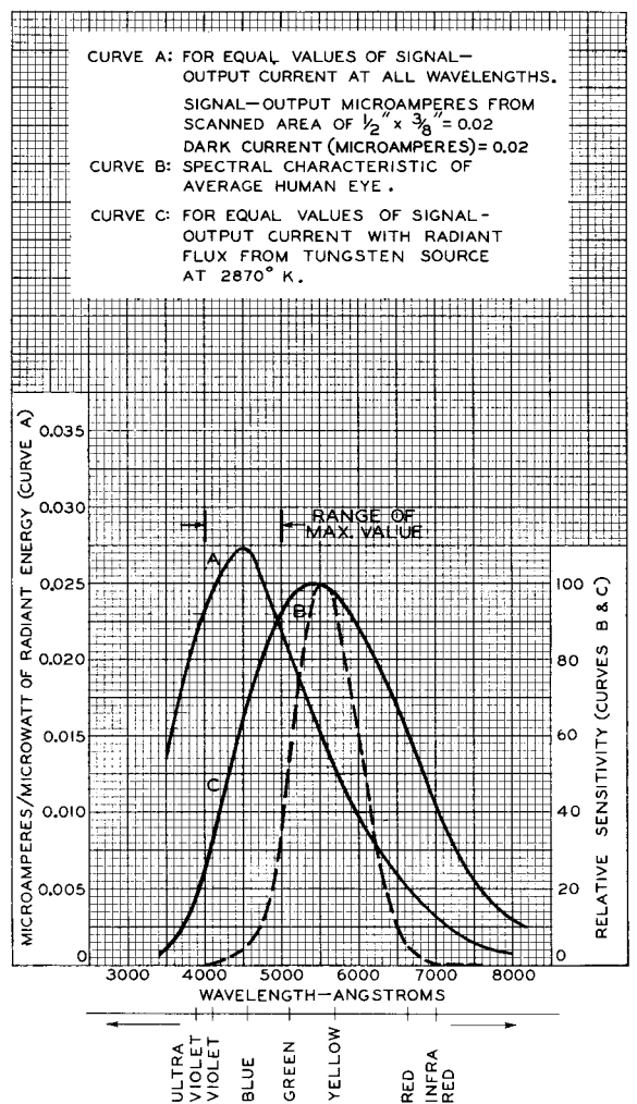
Fig. 12 - Spectral Sensitivity Characteristics of Type 7262.
