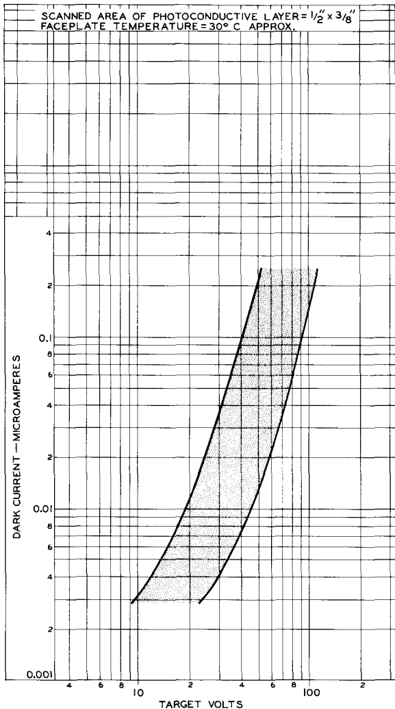
Fig.3 — Range of Dark Current for Type 7262.
