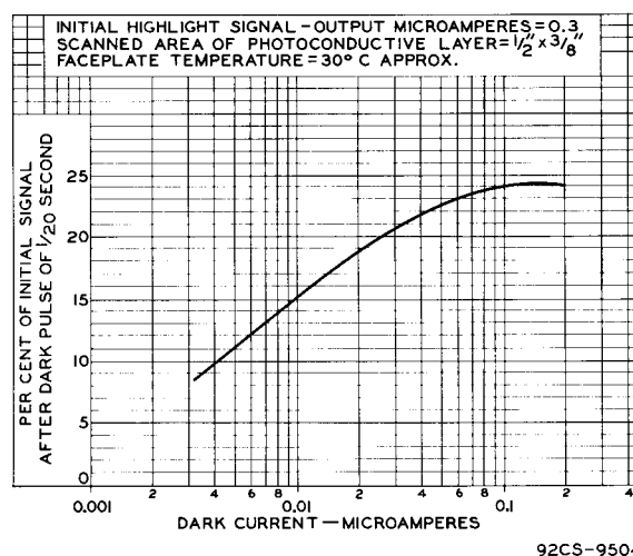
Fig. 11 - Typical Persistence Characteristic of Type 7262.
