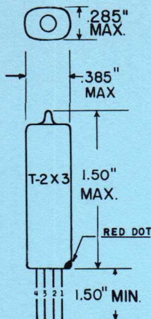
GLASS BULB RED DOT IS ADJACENT TO LEAD 1 IN LINE BASE OUTLINE DRAWING JEDEC 2-1
