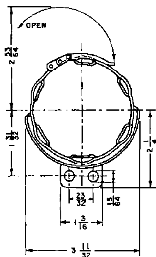
GRID CONNECTOR S-17288
