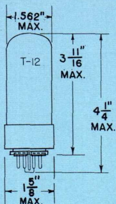
GLASS BULB SMALL WAFER 8 PIN OCTAL BB-197
