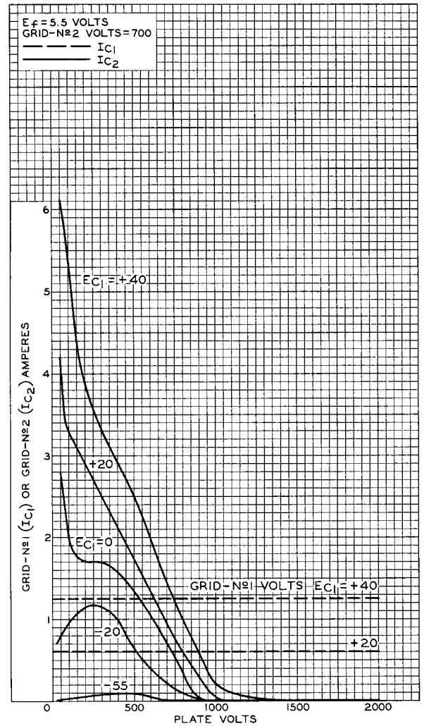
Fig.6 - Typical Characteristics of Type 7213.
