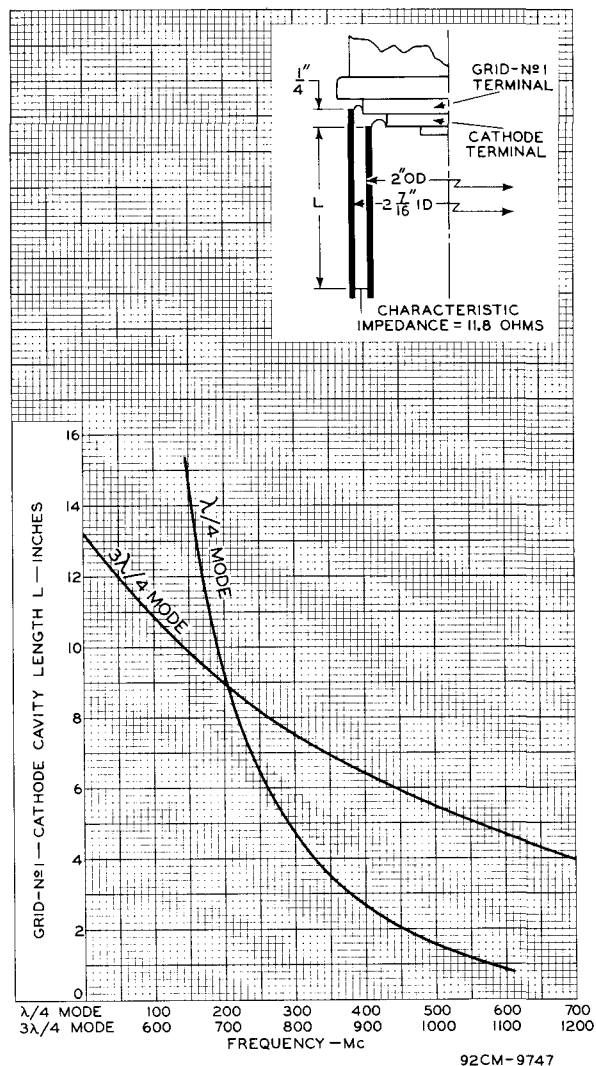
Fig. 10 - Grid No. 1--Cathode Tuning Curves.
