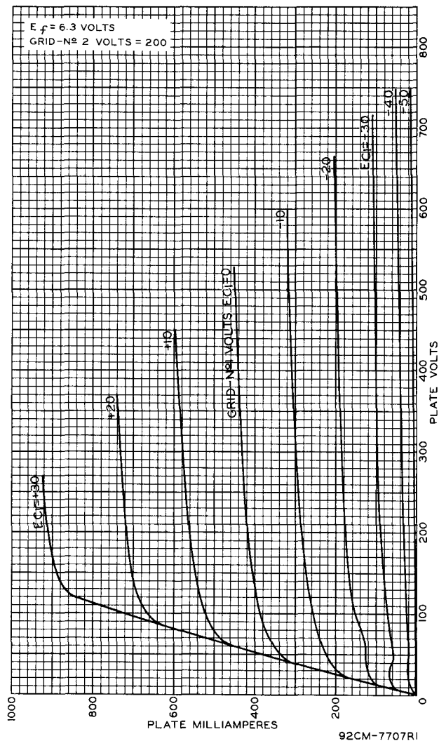
Fig. 4 - Average Plate Characteristics of Type 7212.
