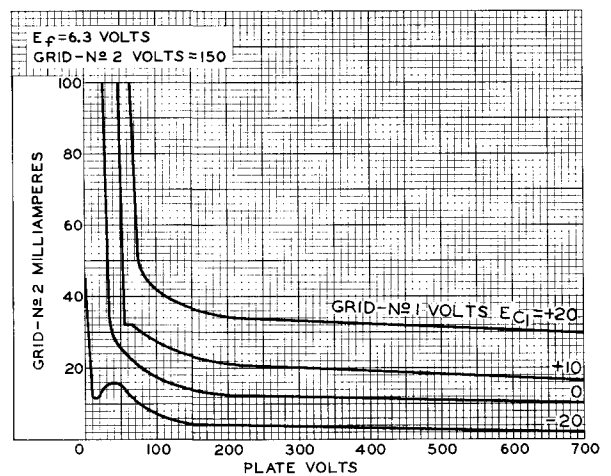
Fig. 3 - Average Characteristics of Type 7212.
