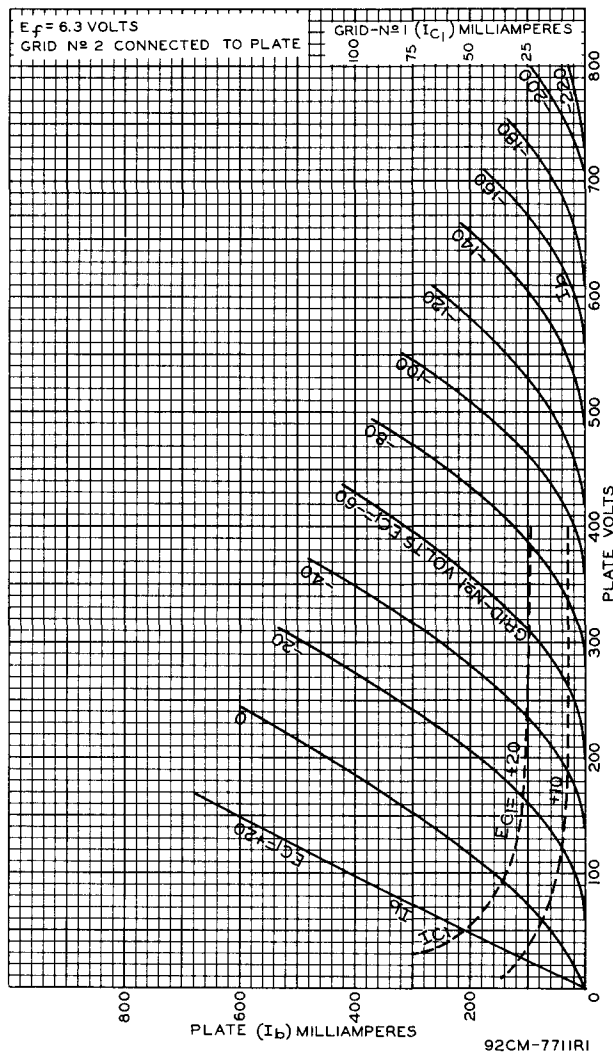
Fig. 7 - Average Characteristics of Type 7212 with Triode Connection.
