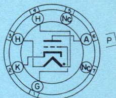
BOTTOM VIEW SMALL BUTTON MINIATURE 7 PIN BASE 7FK
