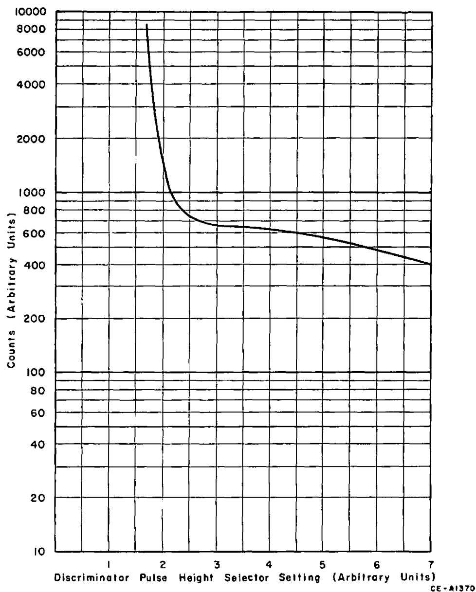
COUNTER SENSITIVITY AS A FUNCTION OF PULSE HEIGHT SELECTOR SETTING
