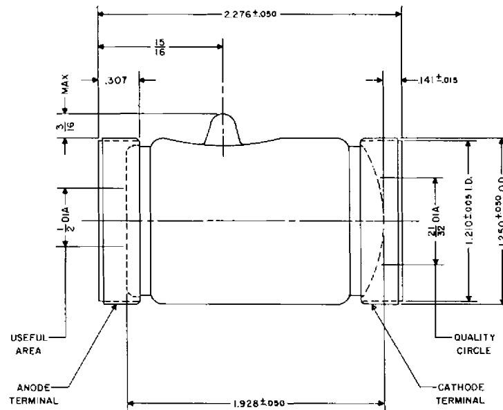
OUTLINE DRAWING
