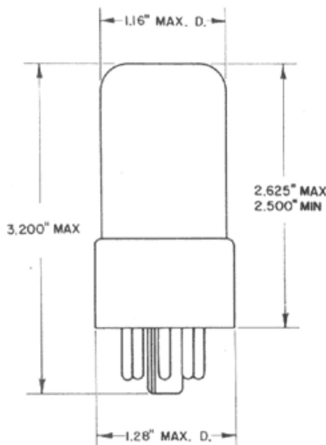
6909 Outline Drawing
