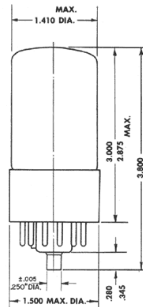
6910 Outline Drawing
