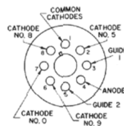
Base Connections
