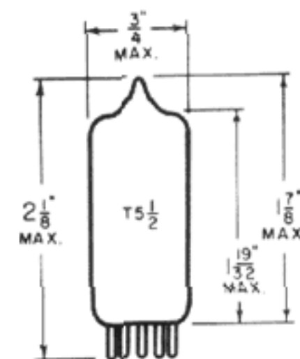
Outline Drawing
