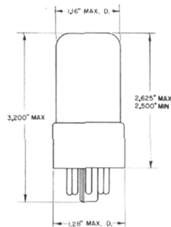
Outline Drawing
