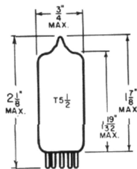
Outline Drawing
