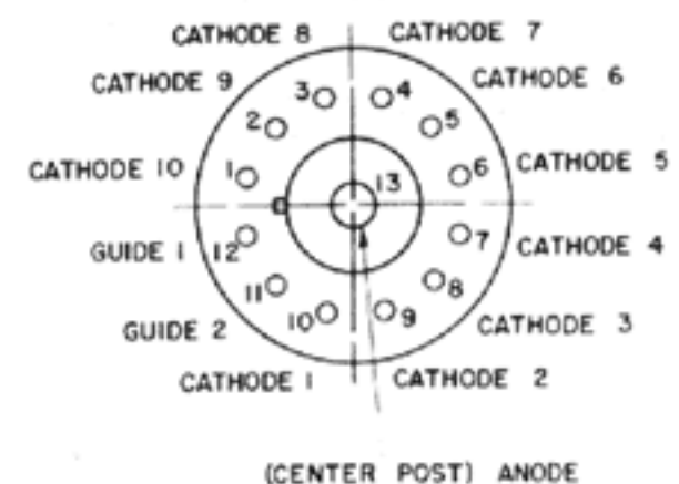
6910 Base Connections
