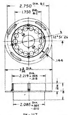
FIG. 9 CONTACT SOCKET ASSEMBLY SK 117 FOR JUMBO TUBES
