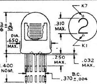
FIG. 3 OUTLINE DRAWING FOR MINIATURE TUBES
