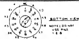
FIG. 5 ENVELOPE CONNECTION DIAGRAM FOR STANDARD SUPER AND JUMBO TUBES
