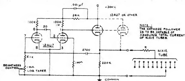
Figure 6—Nixie Tube Dimming Circuit
