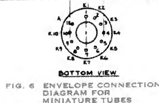
FIG. 6 ENVELOPE CONNECTION DIAGRAM FOR MINIATURE TUBES
