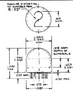
FIG. 1 OUTLINE DRAWING FOR STANDARD TUBES
