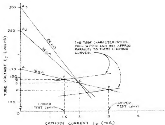
Figure 2—6844A Characteristic Curves
