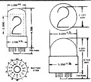
FIG. 4 OUTLINE DRAWING FOR JUMBO TUBES
