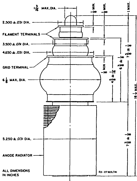
DIMENSIONS — ML-7125
