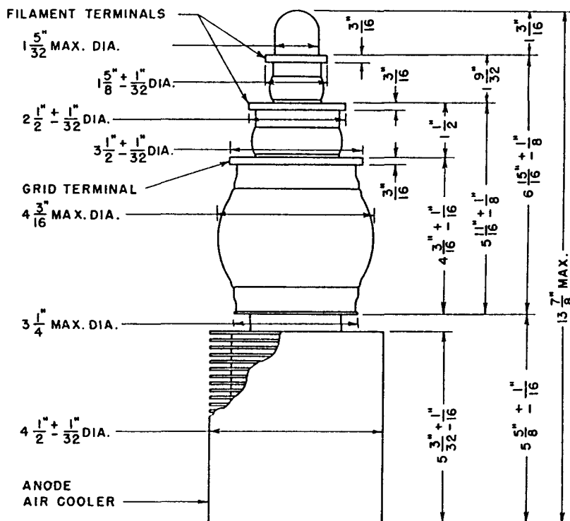
DIMENSIONS — ML-7121
