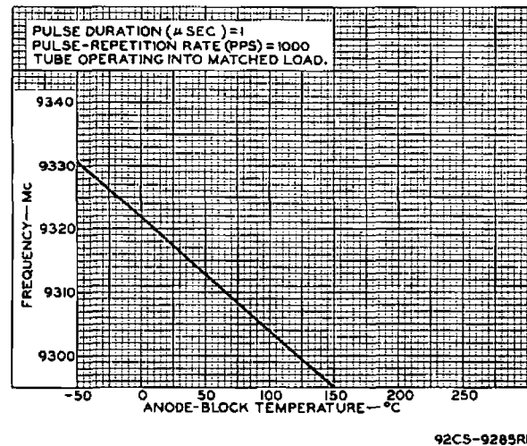
Fig. 3 - Typical Thermal-Factor Characteristics of Types 7110, 7111, and 7112.
