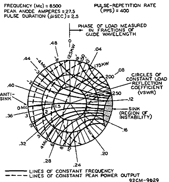
Fig. 6 - Typical Performance Curves for Types 7110, 7111 and 7112.
