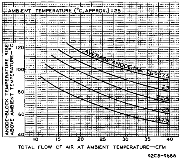
Fig. 1 - Typical Cooling Requirements for Anode Block of Types 7110, 7111, and 7112 with Cooling Arrangement Described in Text.
