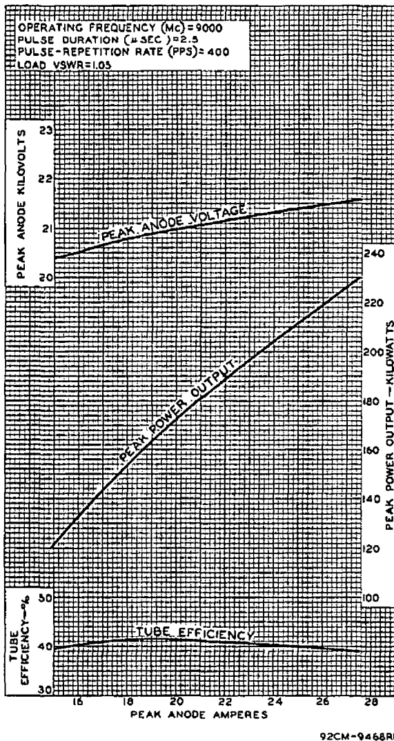
Fig. 5 - Typical Performance Curves for Types 7110, 7111, and 7112.
