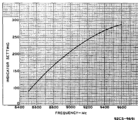
Fig. 8 - Representative Tuning Characteristic of Types 7110, 7111, and 7112.
