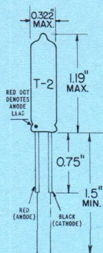
GLASS BULB
