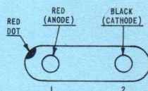
BOTTOM VIEW FLAT PRESS WITH 2 FLYING LEADS
