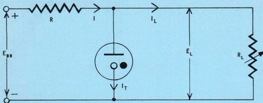
TYPICAL CIRCUIT FOR VOLTAGE REGULATOR
