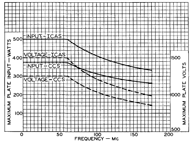
Rating Chart II for Type 7094 in Class C Telephony Service.
