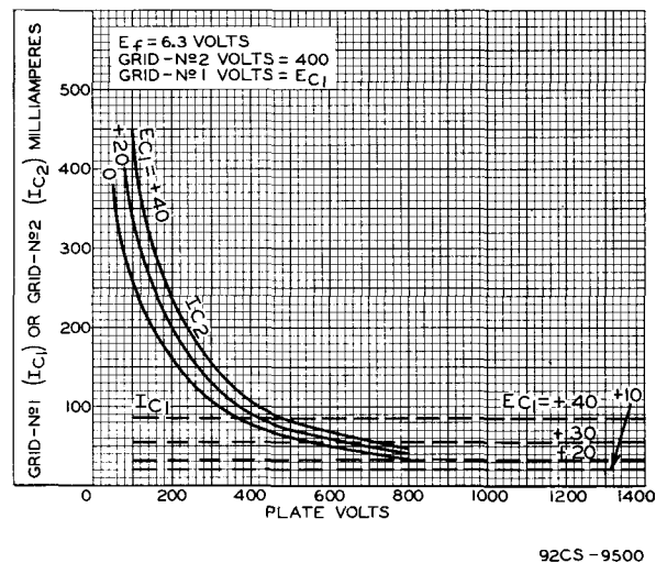
Fig. 4 - Typical Characteristics for Type 7094.
