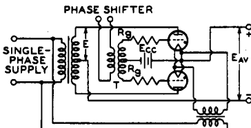
FIG. 4 FULL-WAVE SINGLE-PHASE
