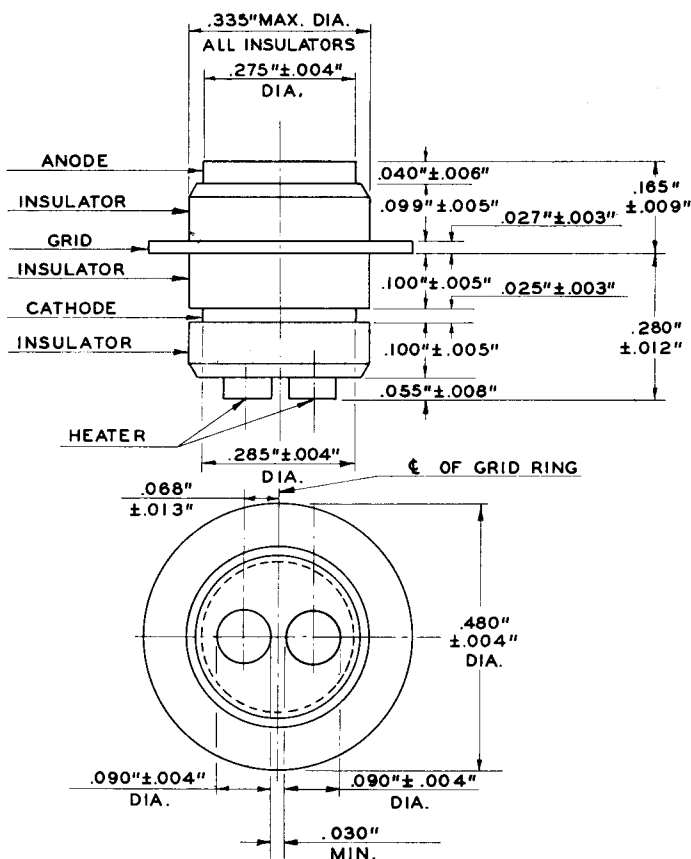
OUTLINE DRAWING
