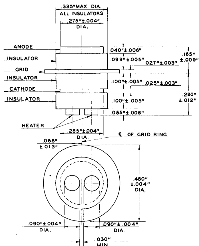
OUTLINE DRAWING
