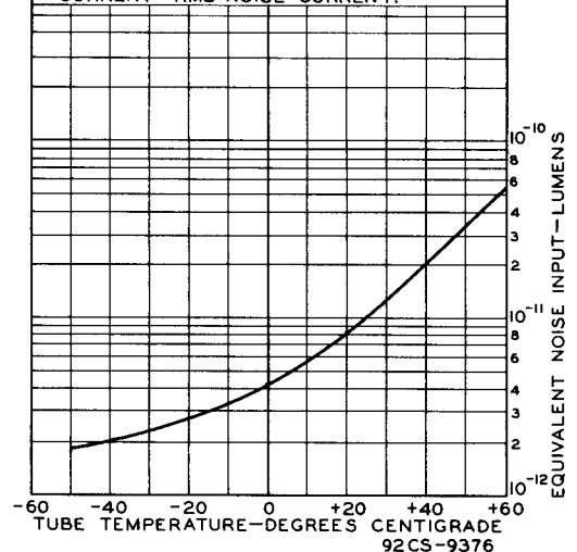
Fig.7 - Equivalent-Noise-Input Characteristic of Type 7046.
