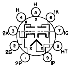
BASING DIAGRAM
