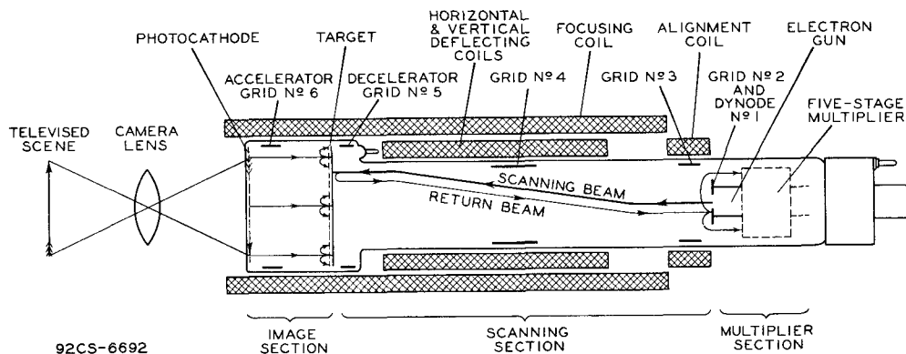
Fig.2 - Schematic Arrangement of Type 7037.
