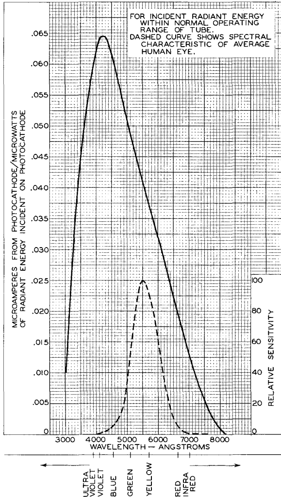
Fig. 1 - Spectral Sensitivity Characteristic of Type 7037.
