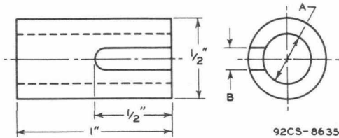
GAUGE SKETCH G 2
