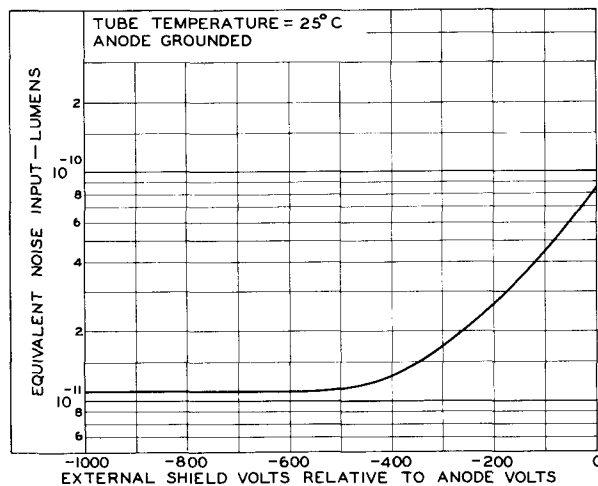
Fig. 7 - Effect of External-Shield Potential on Equivalent Noise Input of Type 7029.
