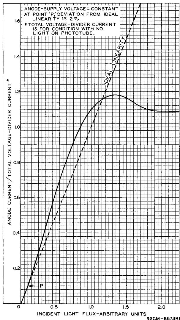
Fig.9 - Linearity Characteristic of Type 7029 as Affected by Ratio of Anode Current to Total Divider Current.
