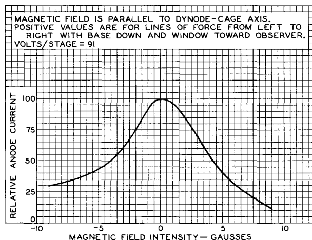
Fig. 8 - Effect of Magnetic Field on Anode Current of Type 7029.
