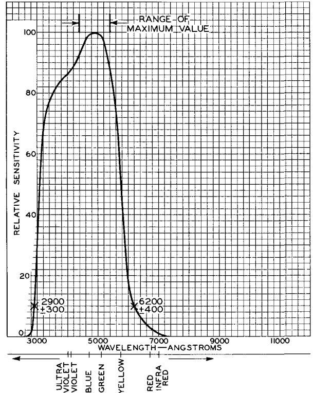
Fig. 1 - Tentative Spectral Sensitivity Characteristic of Type 7029 which has S-17 Response.
