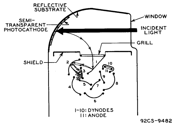
Fig. 3—Schematic Arrangement of Type 7029.
