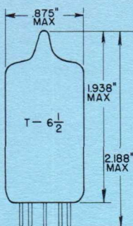
GLASS BULB SMALL BUTTON 9 PIN BASE E9-1 OUTLINE DRAWING JEDEC 6-2
