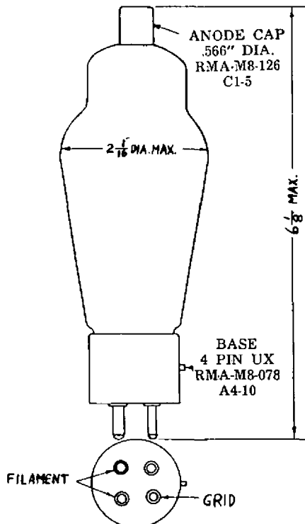
OUTLINE DRAWING
