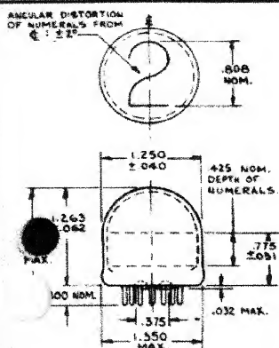
FIG. 2 OUTLINE DRAWING FOR SUPER TUBES
