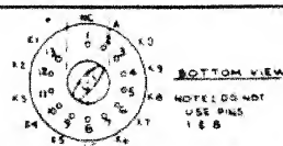
FIG. 5 ENVELOPE CONNECTION DIAGRAM FOR STANDARD SUPER AND JUMBO TUBES
