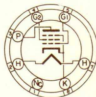
BOTTOM VIEW SHORT MEDIUM SHELL 7 PIN OCTAL
