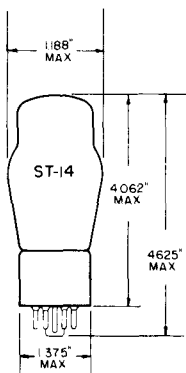
GLASS BULB MEDIUM SHELL 7 PIN OCTAL B7-12 JEDEC 14-3
