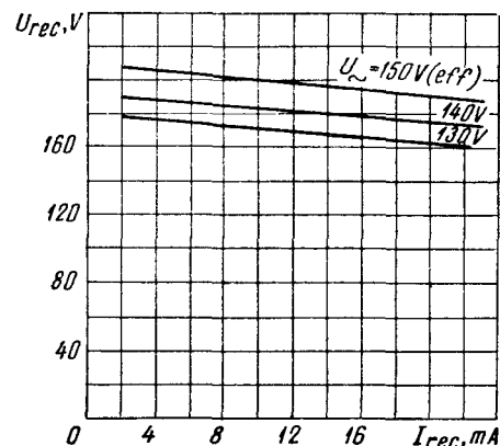
U_{rec} = f(I_{rec}) U_h = 6,3 V C_{\text{фильтра}} = 8 \mu F R_a^{1)} = 200 \Omega filter
