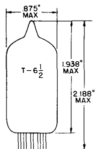
GLASS BULB MINIATURE GLASS BUTTON 9 PIN BASE E9-1 OUTLINE DRAWING JEDEC 6-2
