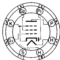
BOTTOM VIEW SMALL WAFER 8 PIN OCTAL 7A2
