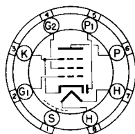
BOTTOM VIEW SMALL WAFER 8 PIN OCTAL 7AZ
