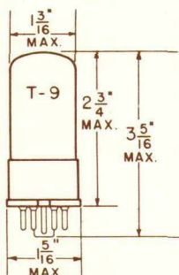
GLASS BULB
